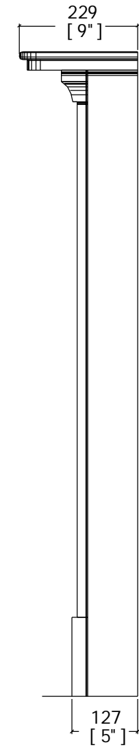
SIDE ELEVATION
