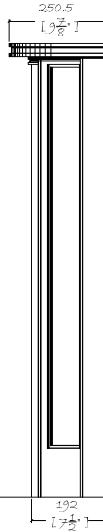
SIDE ELEVATION
