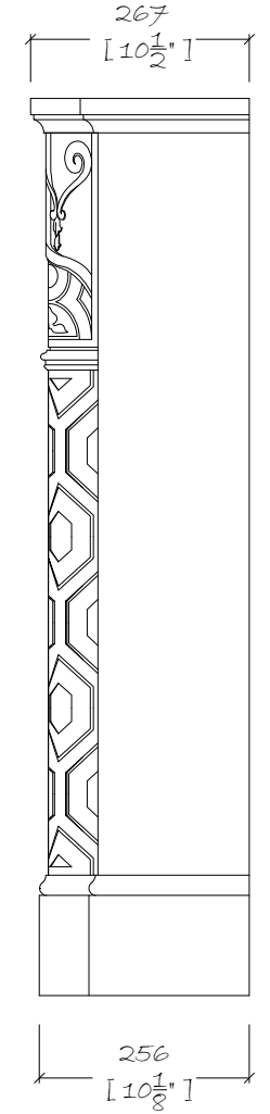
SIDE ELEVATION
