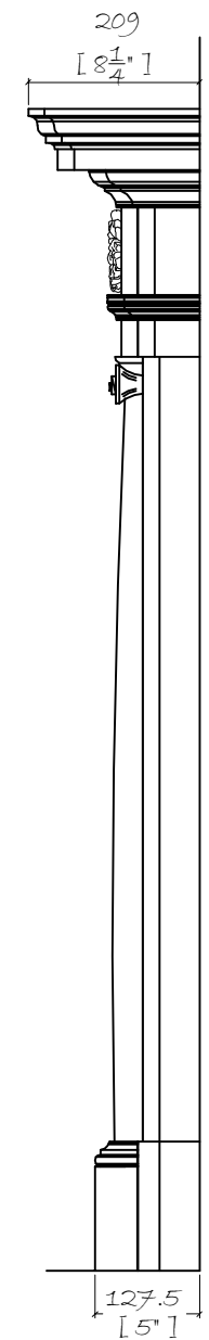
SIDE ELEVATION
