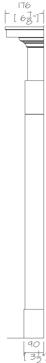
SIDE ELEVATION
