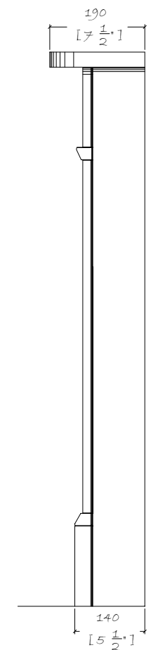
SIDE ELEVATION
