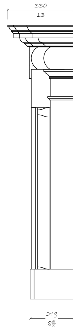
SIDE ELEVATION
