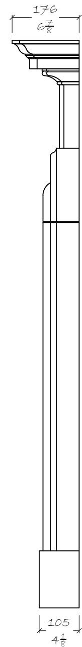
SIDE ELEVATION
