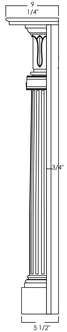
SIDE ELEVATION
