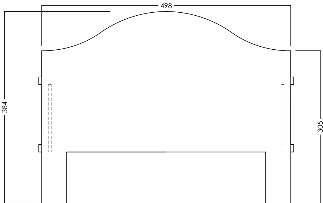
REAR ELEVATION
