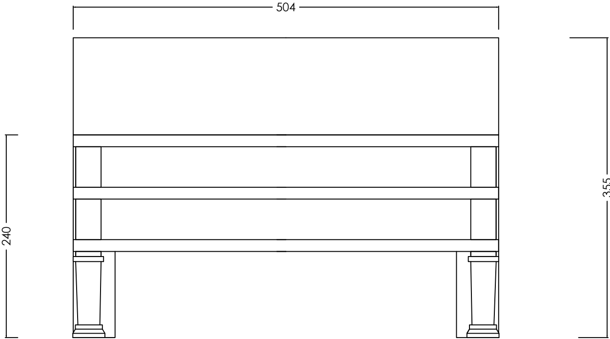
FRONT ELEVATION
