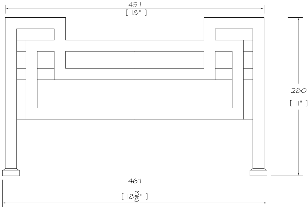
FRONT ELEVATION
